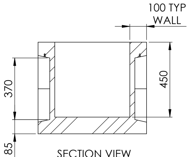
450 x 450 x 450 CONCRETE PIT WEIGHT = 350 kg
