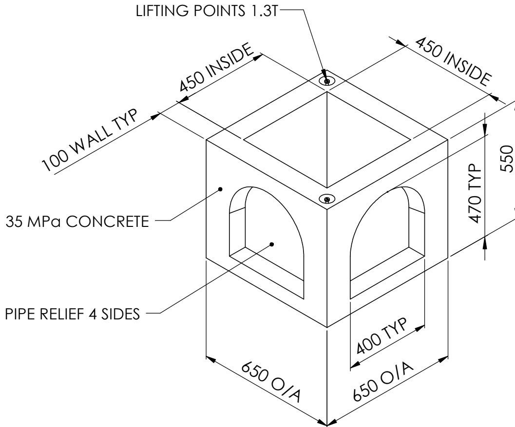
450 x 450 x 450 CONCRETE PIT WEIGHT = 350 kg
