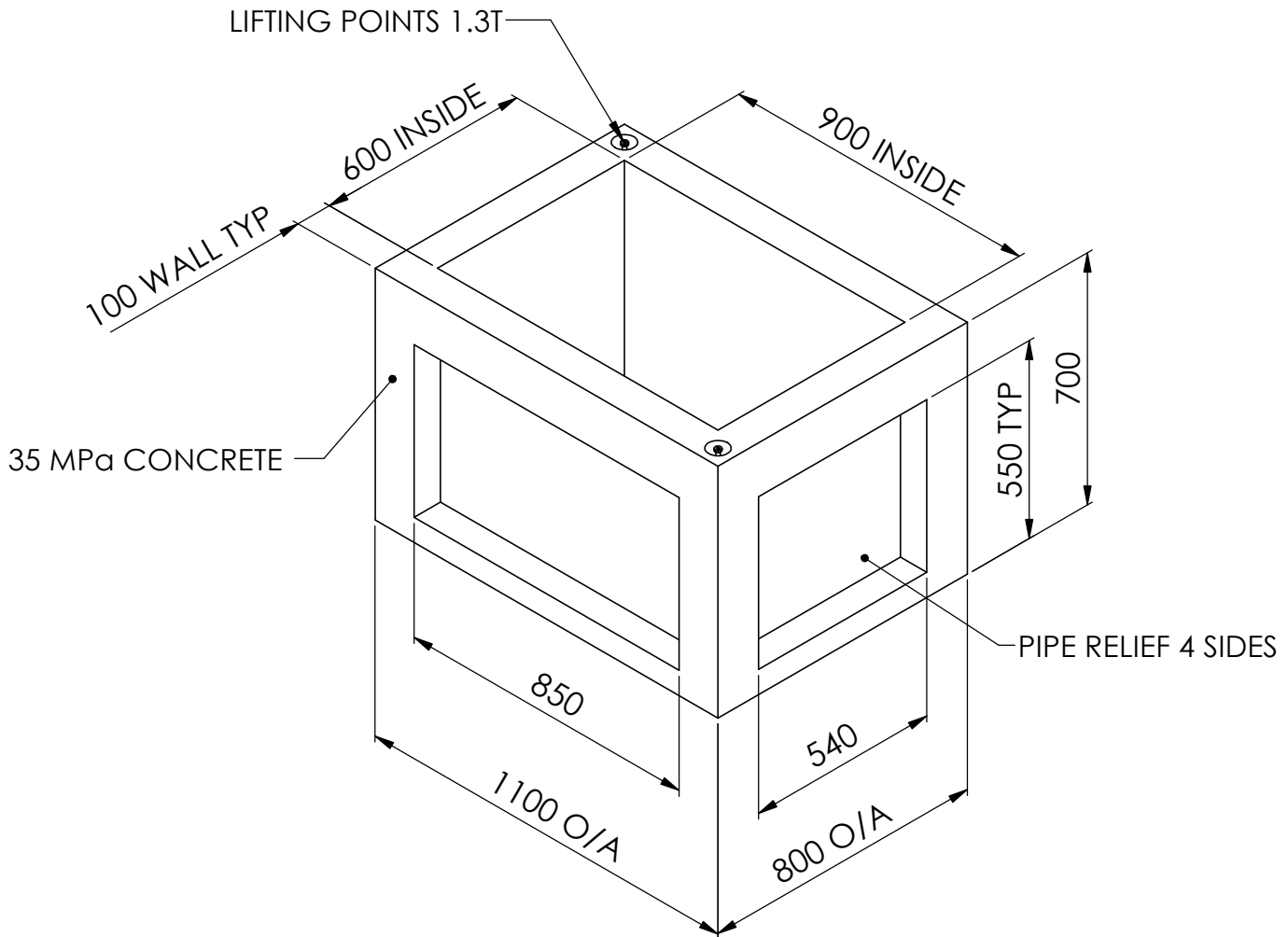
900 x 600 x 600 CONCRETE PIT WEIGHT = 500 kg
