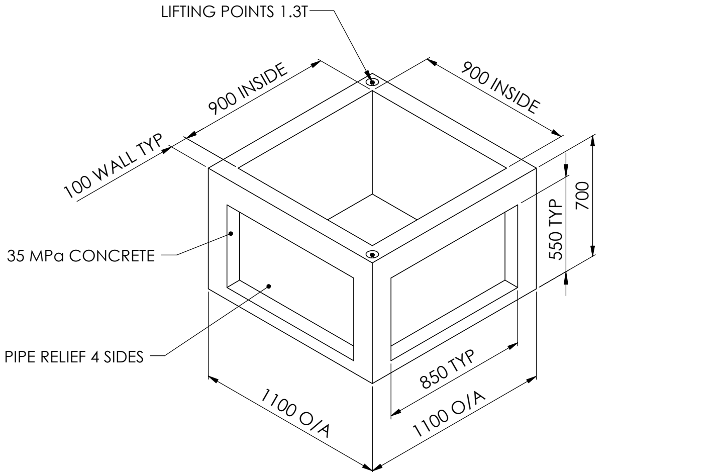
900 x 900 x 600 CONCRETE PIT WEIGHT = 625 kg
