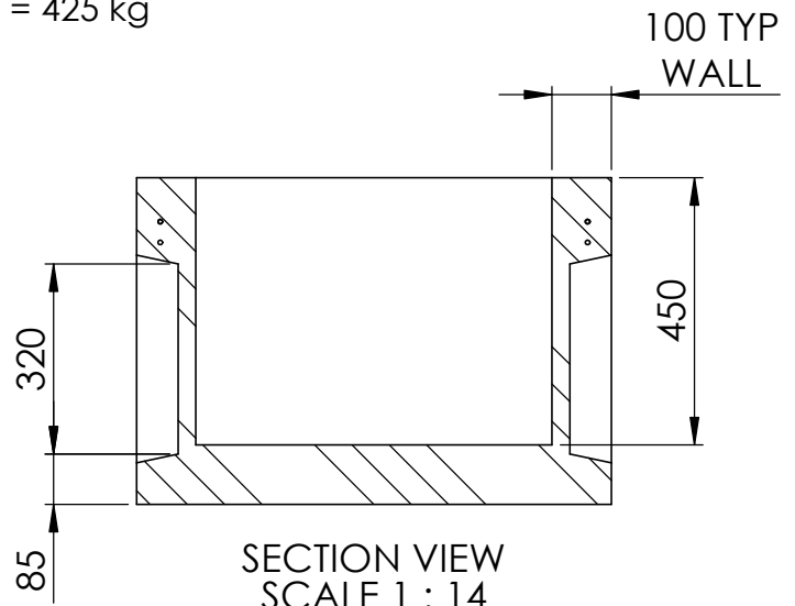
600 x 600 x 450 CONCRETE PIT WEIGHT = 425 kg
